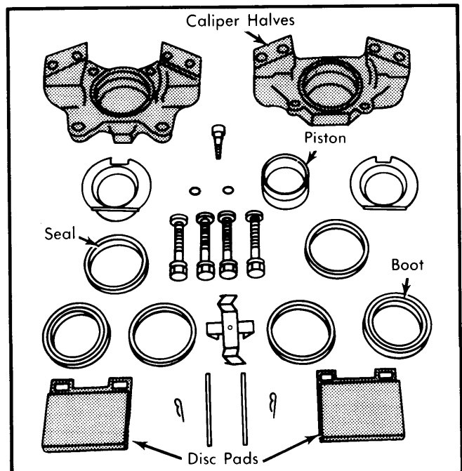
Fig. 5 Disassembled View of Typical Mercedes-Benz Brake Caliper
