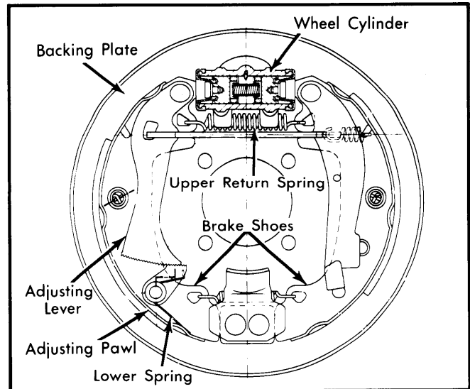
Fig. 4 Brava Rear Drum Brake Assembly
