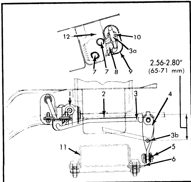
Fig. 3 Brake Pressure Regulator Measurement and Adjustment Points for Strada Models
