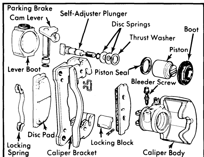
Fig. 8 Exploded View of Rear Brake Caliper Spider 2000 Shown - X1/9 Similar
