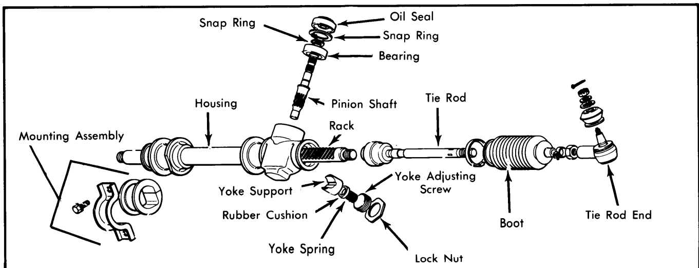
Fig. 1 Exploded View of Champ and Colt Hatchback Rack and Pinion Steering
