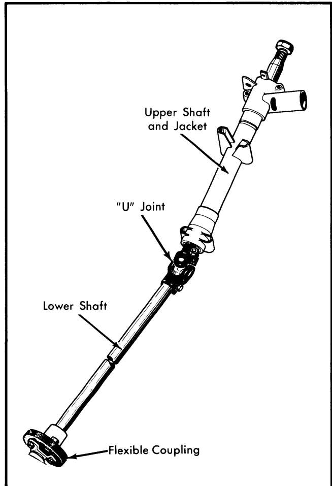
Fig. 2 Peugeot Steering Column Assembly (504 Shown, 505 and 604 Similar)
