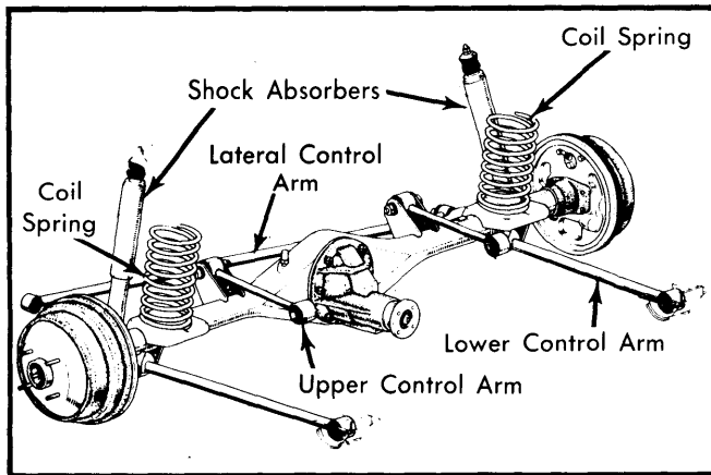
Fig. 1 Rear Suspension Arrangement of Toyota Celica & Cressida (Supra Similar)
