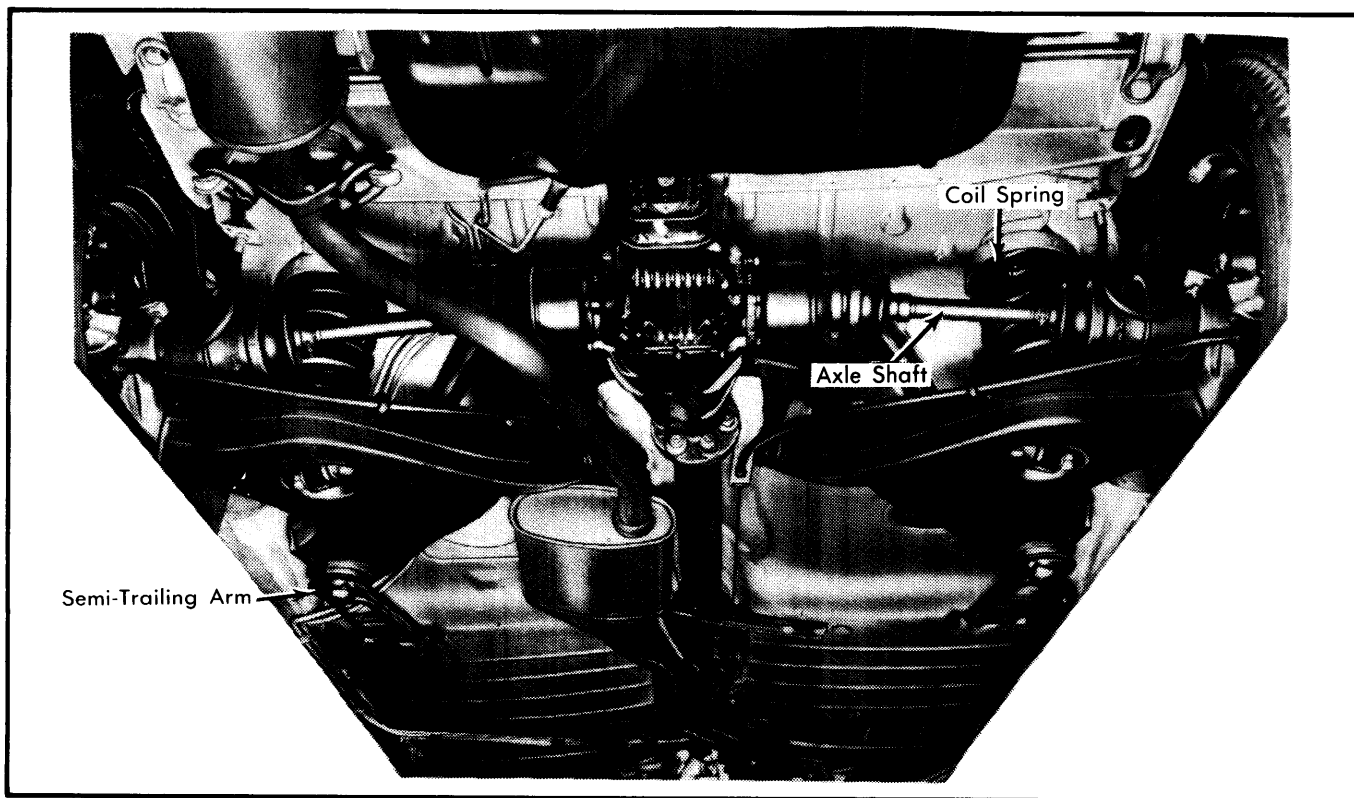
Fig. 2 Rear to Front View of Typical Mercedes Benz Rear Suspension
