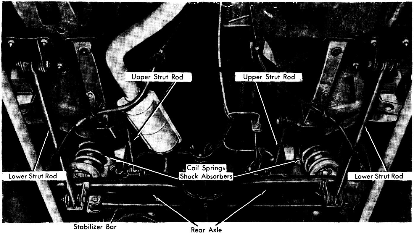
Fig. 1 Installed View of Fiat Spider 2000 Rear Suspension Assembly
