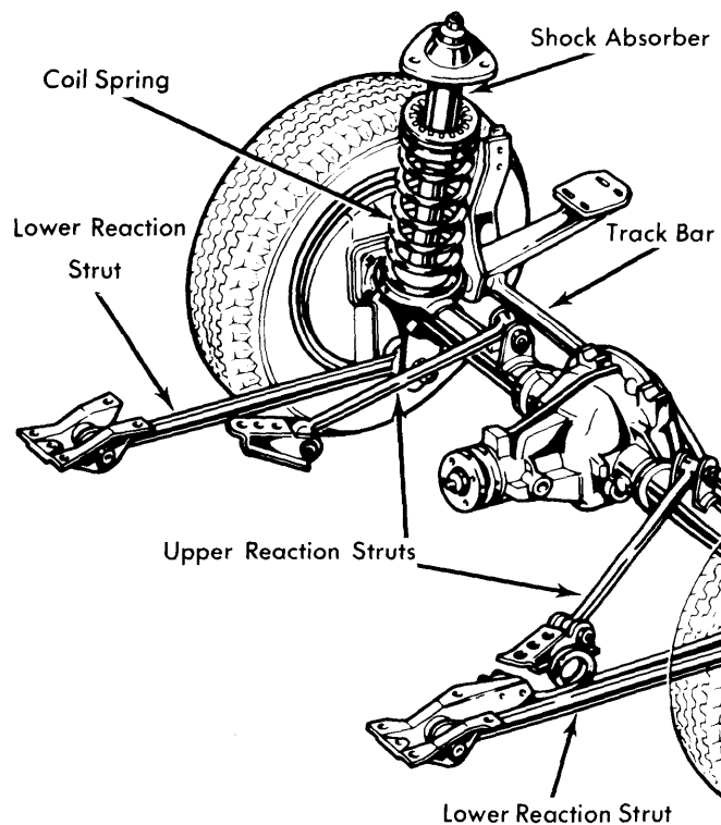
Fig. 1 Fiat Brava Rear Suspension Assembly (Sedan Shown; Station Wagon Similar)
