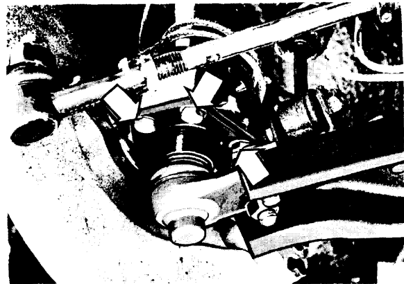
Fig. 4 View Showing Ball Joint Retaining Bolts
