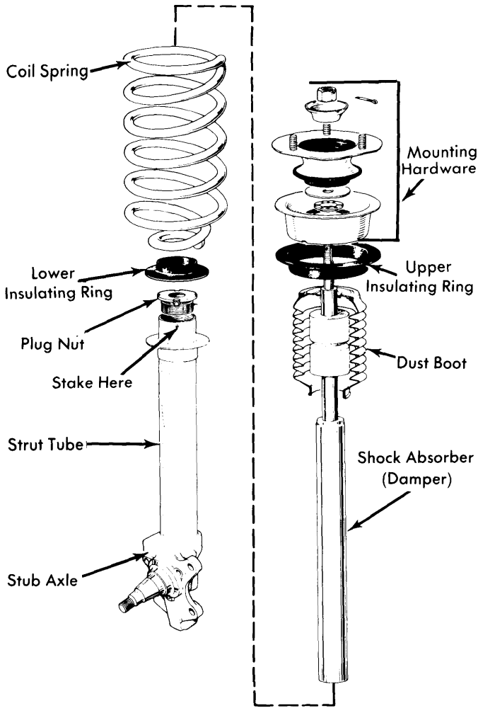
Fig. 3 Disassembled View of Strut
