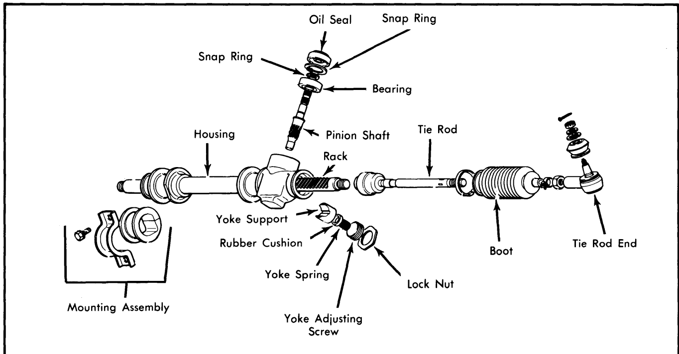
Fig. 1 Exploded View of Champ & Colt (FWD) Rack & Pinion Steering
