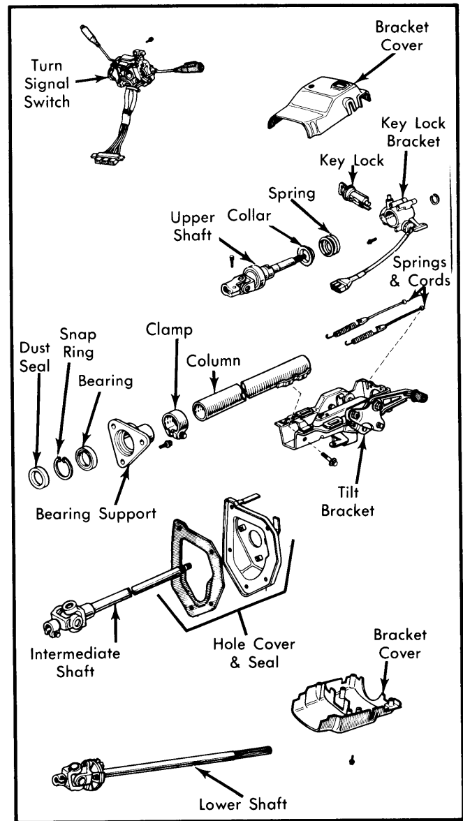
Fig. 2 Exploded View of Pickup Tilt Wheel Steering Column
