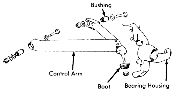
Fig. 2 Exploded View of Control Arm Assembly
