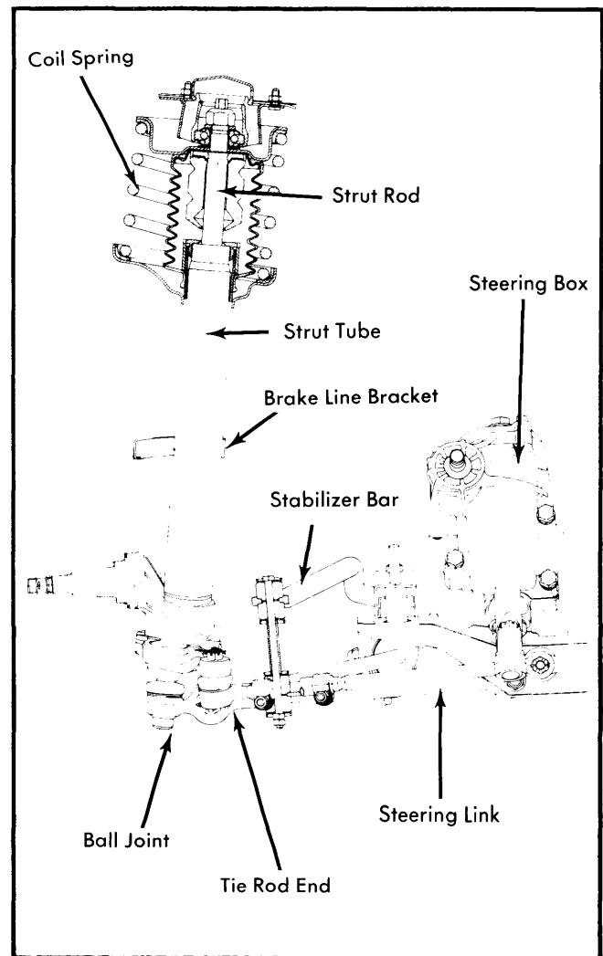
Fig. 2 BMW 530i, 633CSi and 733i Front Suspension
