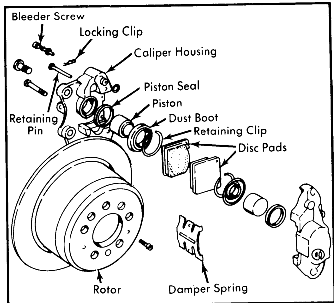
Fig. 6 Girling Rear Caliper
