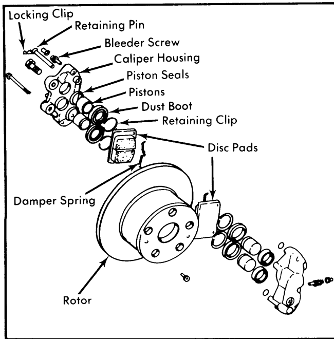
Fig. 5 Girling Front Caliper Assembly
