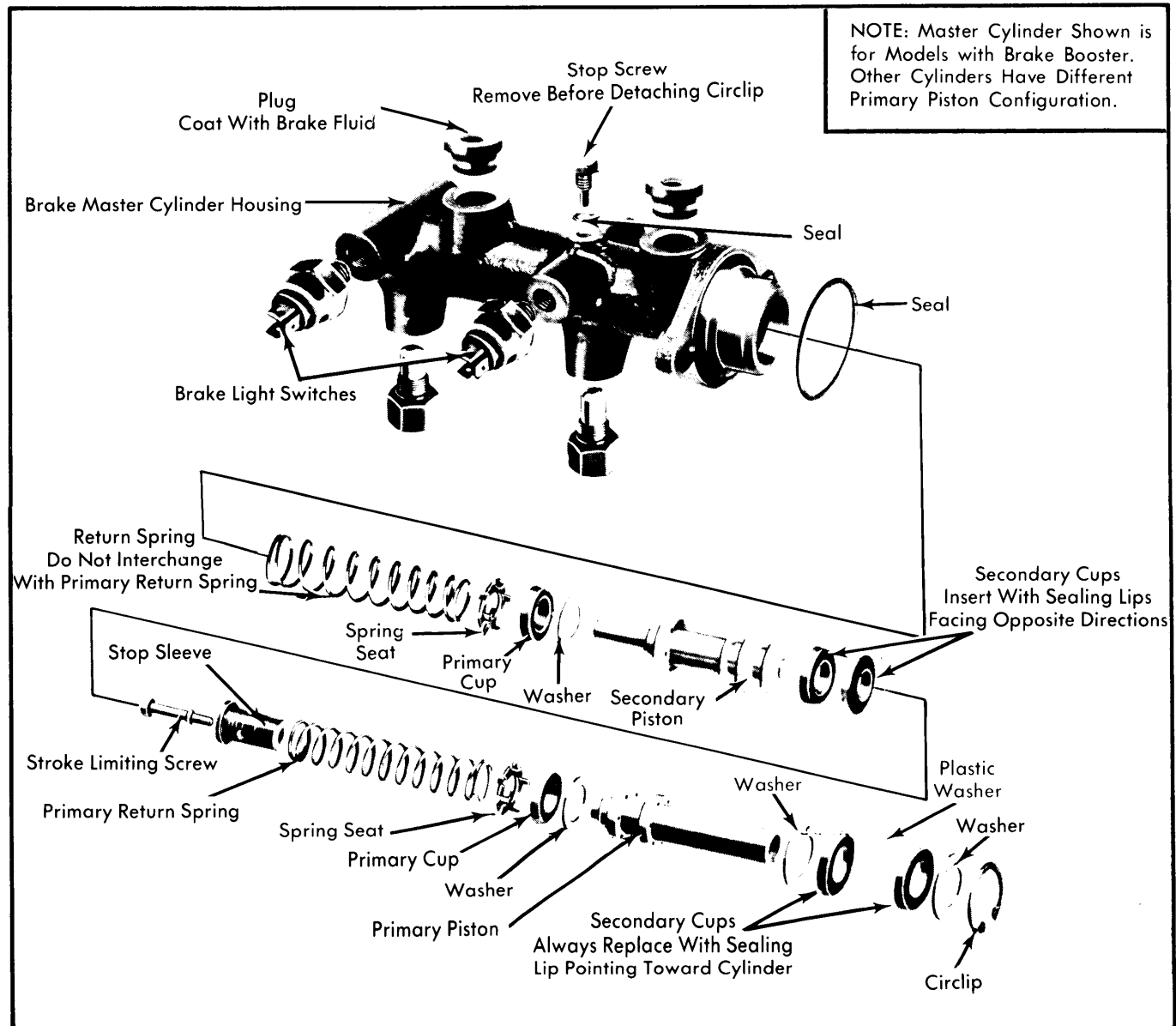
Fig. 10 Master Cylinder Component Relationship - Rabbit, Scirocco, Dasher Shown
