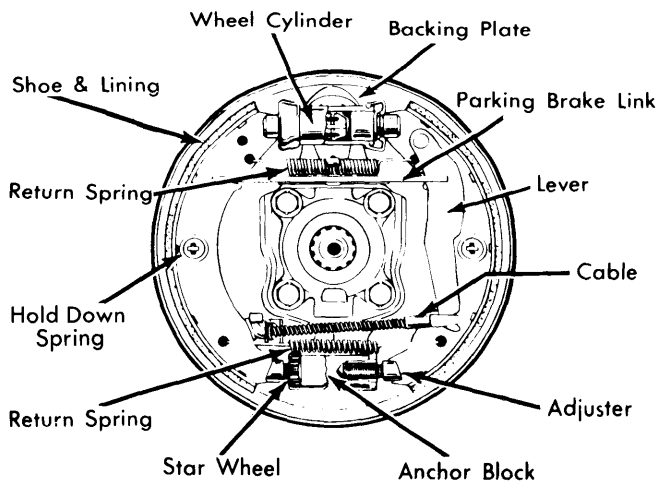
Fig. 5 Volkswagen Type 1 & 2 Rear Brake Assembly with Brake Drum Removed
