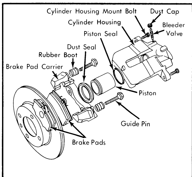
Fig. 8 Exploded View of Girling Disc Brake Assembly Used on Dasher
