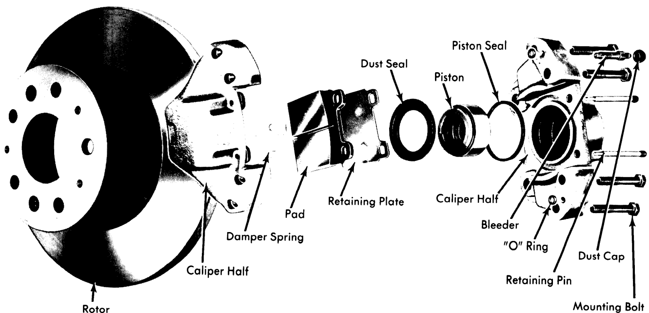
Fig. 3 Volkswagen Type 2 ATE Front Disc Brake Assembly. Girling Caliper Internal Design is Only Slightly Different. Girling Has a Retainer Ring for Dust Seal that is not Integral with Seal.
