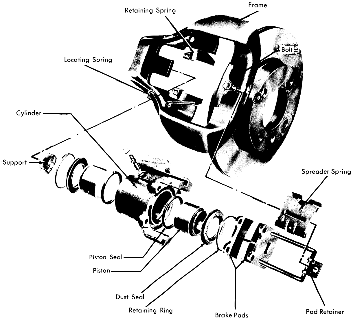
Fig. 7 Exploded View of Girling Disc Brake Assembly Used on Rabbit and Scirocco
