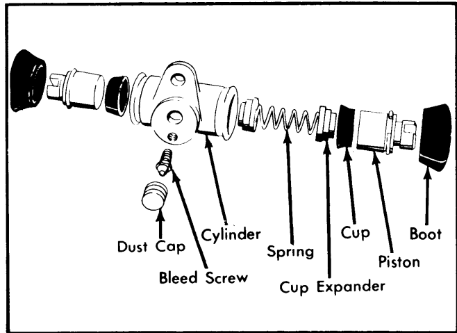
Fig. 9 Volkswagen Type 1 Wheel Cylinder Assembly
