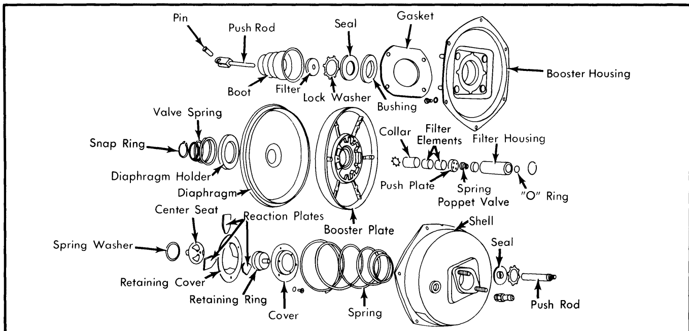
Fig. 7 Exploded View of Civic CVCC Power Booster Unit
