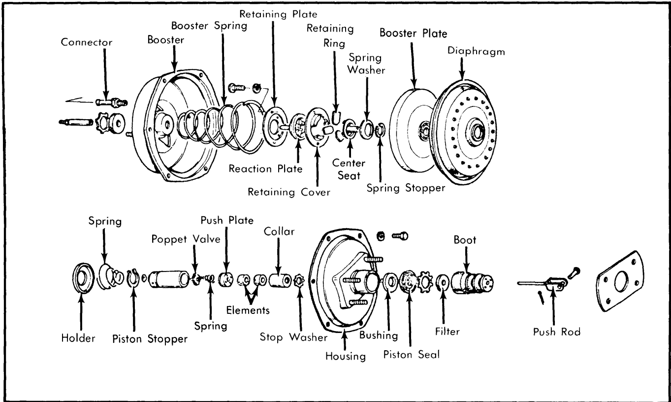
Fig. 8 Exploded View of Honda Civic Power Booster Unit
