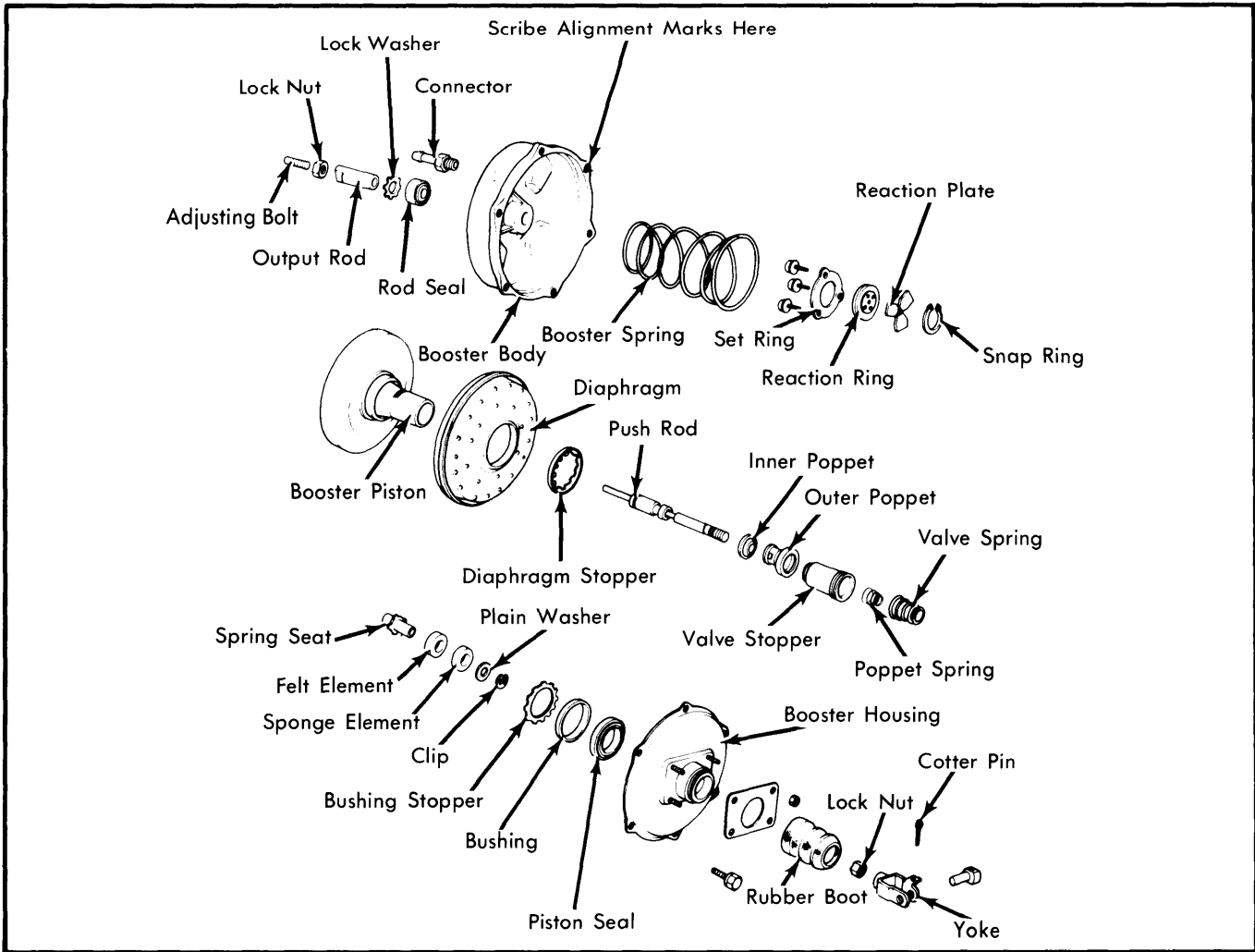
Fig. 6 Exploded View of Honda Accord Power Brake Unit
