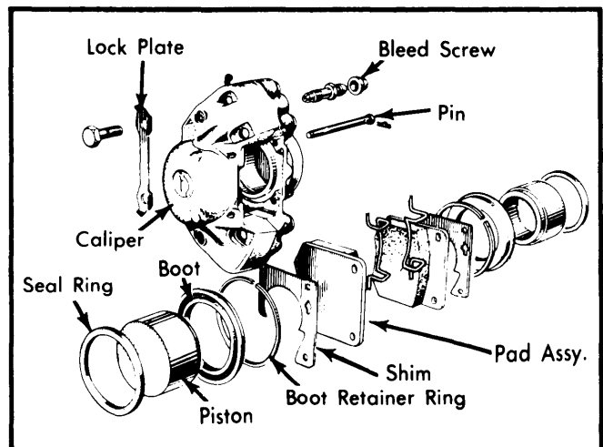
Fig. 2 Exploded View of Front Disc Brake Assy.
