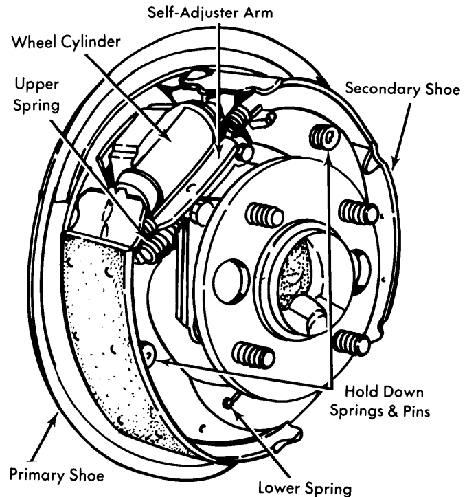
Fig. 3 Assembled View of Rear Drum Brake Components
