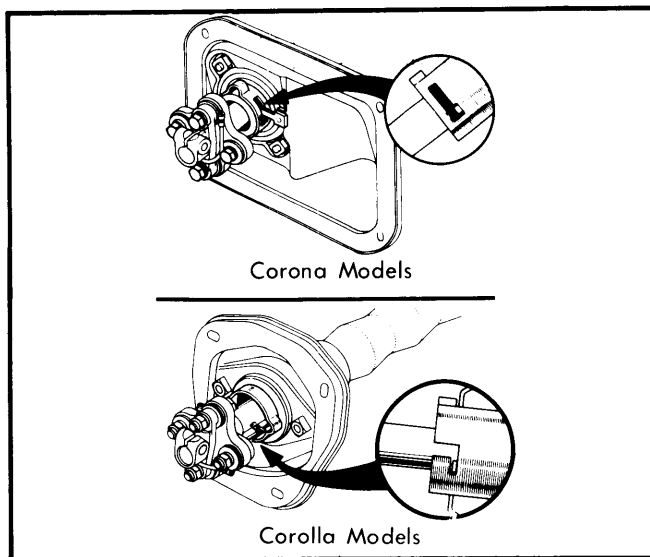
Fig. 3 Proper Installation of Steering Column Locating Pin
