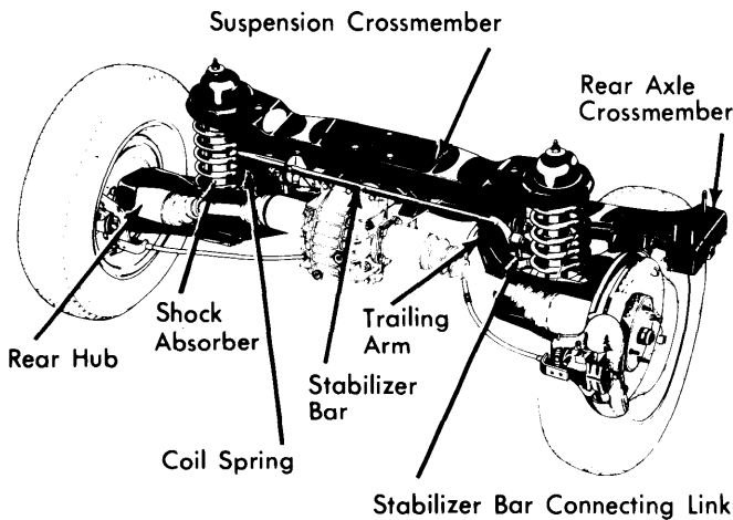
Fig. 1 Peugeot 504 Rear Suspension
