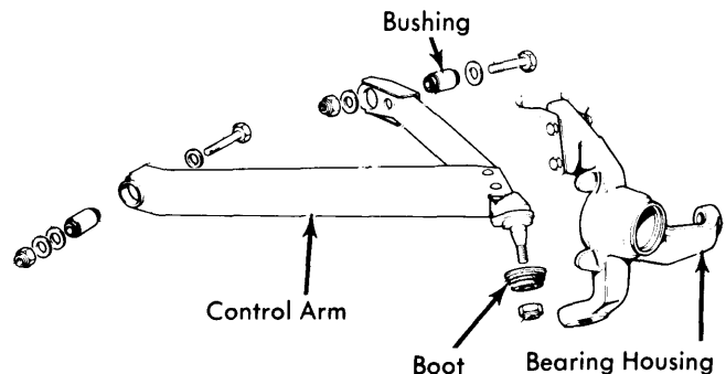
Fig. 2 Exploded View of Control Arm Assembly
