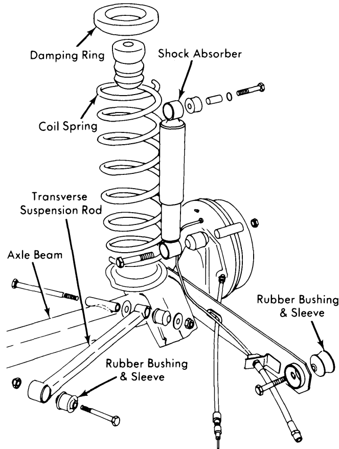
Fig. 1 Exploded View of Fox Rear Suspension
