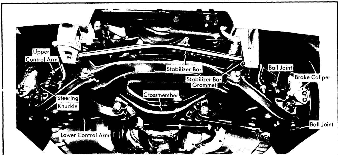
Fig. 2 Head on View of Mercedes-Benz 280 Front Suspension
