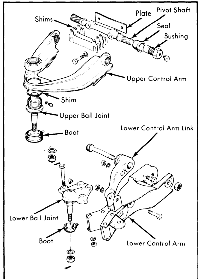
Fig. 1 Exploded View of LUV Front Suspension
