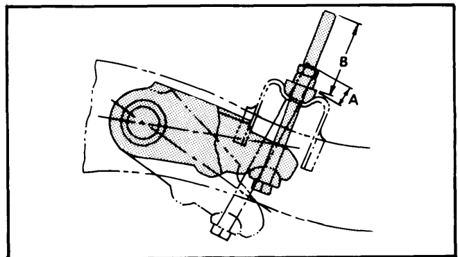
Fig. 2 View Showing Measuring Points for Installation of Anchor Pin
