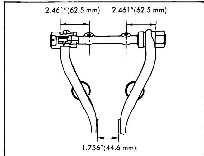
Fig. 4 Measurements for the Upper Control Arm Installation
