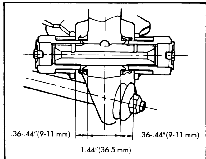
Fig. 5 Measurements for Lower Control Arm Installation
