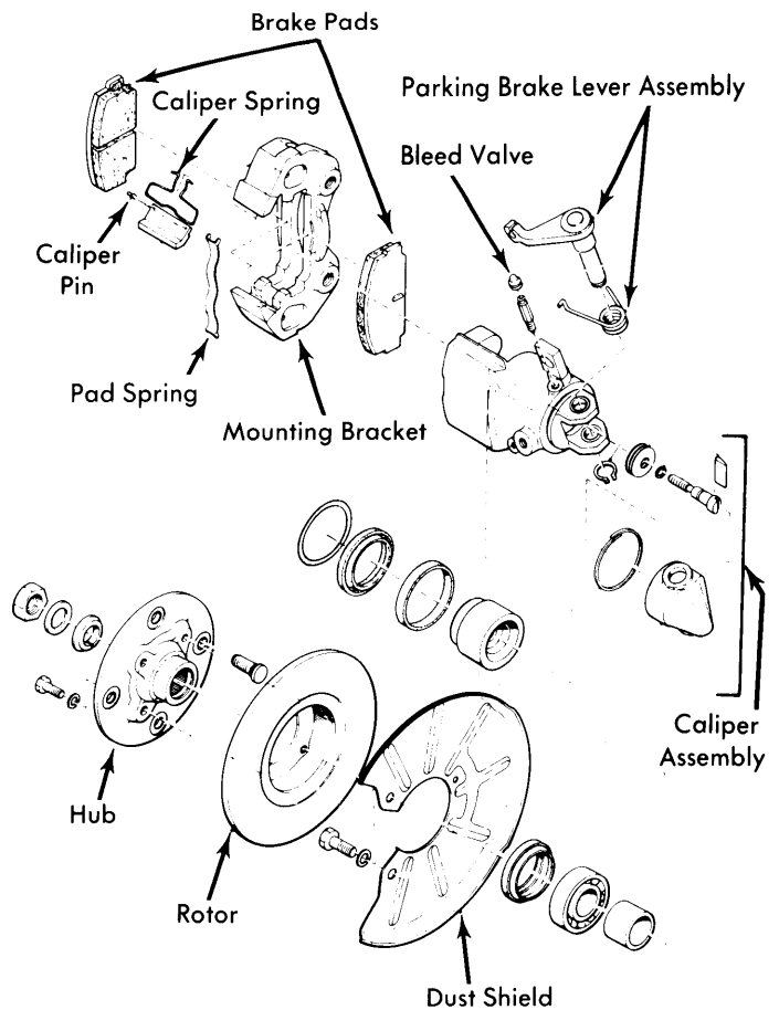
Fig. 1 Exploded View of Front Disc Brake Assembly
