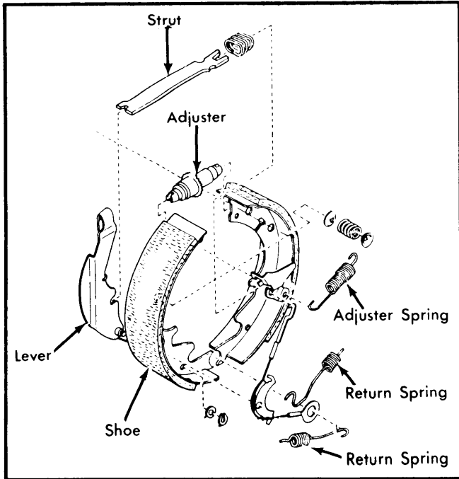
Fig. 2 Exploded View of Front Drum Brake Assembly
