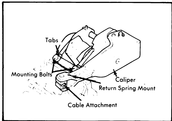
Fig. 1 Detail of Parking Brake Caliper
