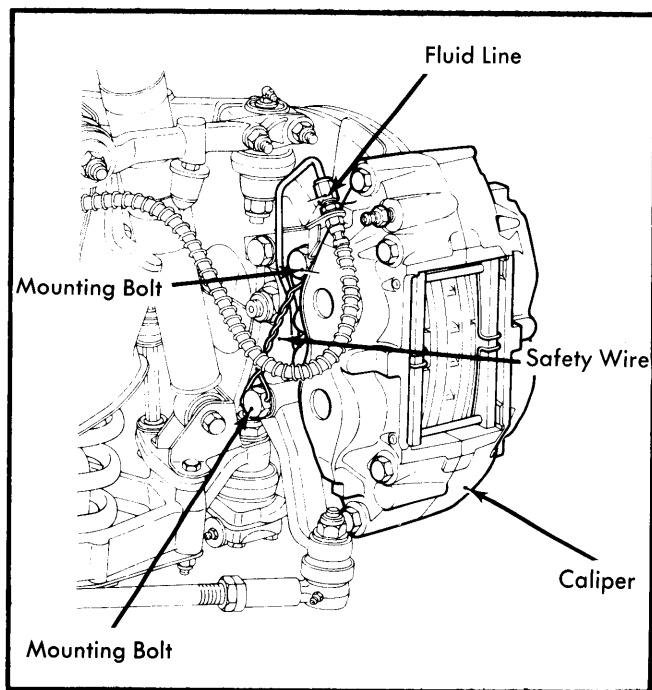
Fig. 2 Components to Remove to Take Off Caliper
