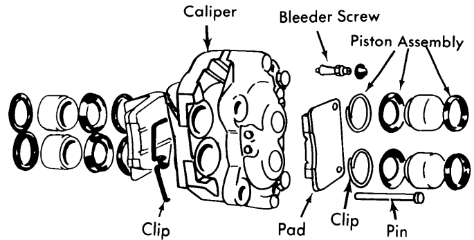
Fig. 3 Exploded View of Front Four Piston Caliper Assembly
