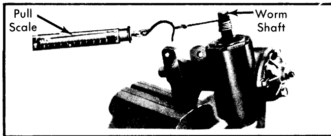
Fig. 3 Measuring Worm Bearing Preload
