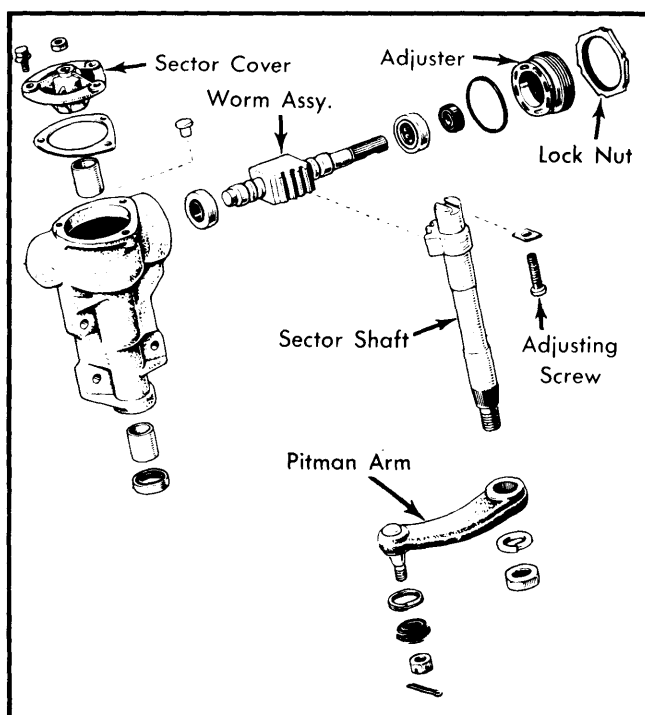
Fig. 2 Exploded View of Recirculating Ball Type Steering (Corona Shown, Others Similar)
