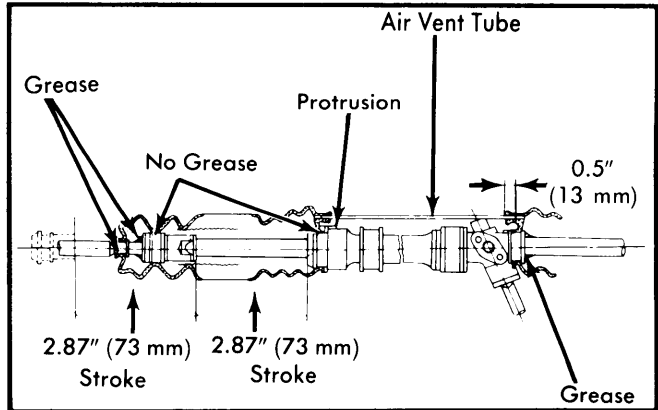
Fig. 4 View Showing Operation Checks and Lubrication of Steering Gear Assembly
