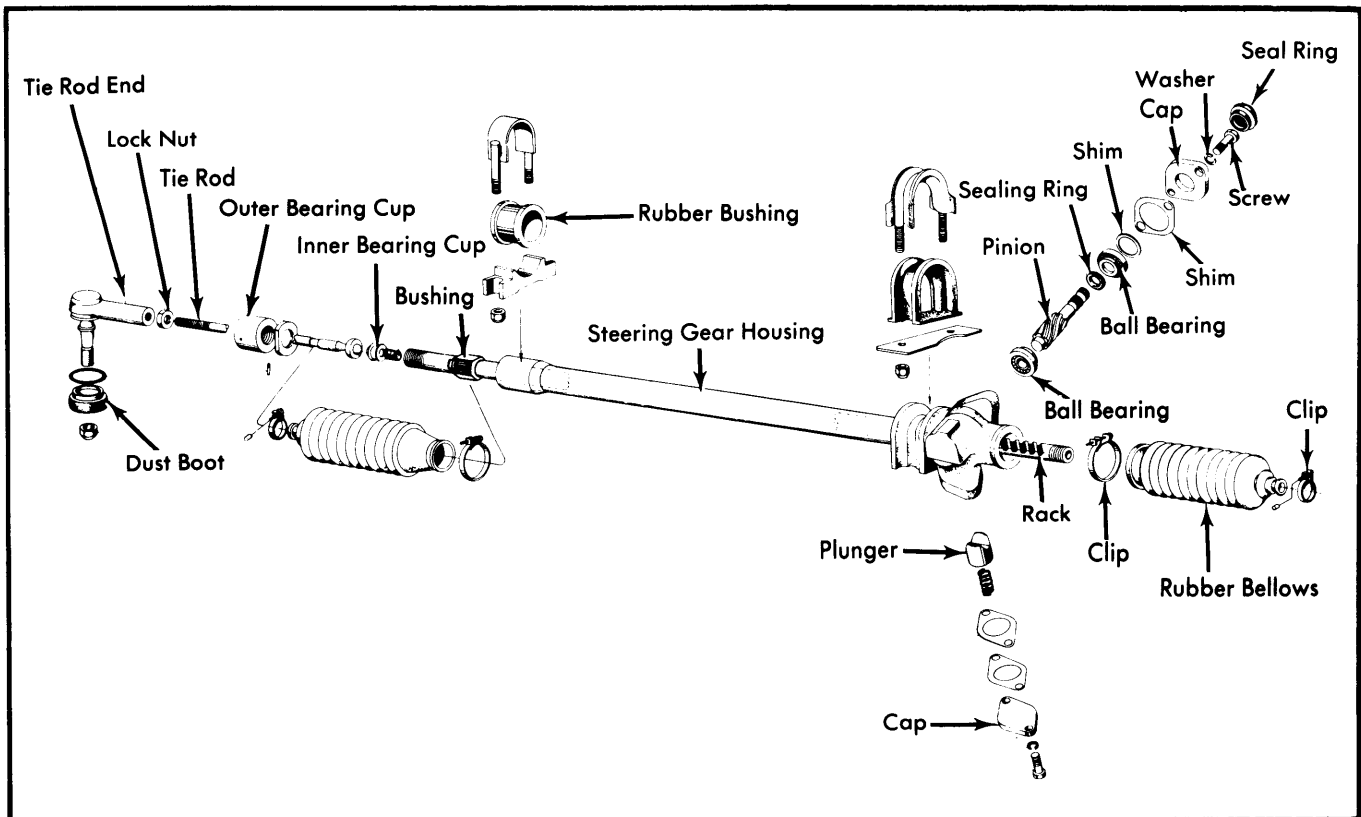
Fig. 2 Exploded View of Saab Rack & Pinion Steering Gear Assembly
