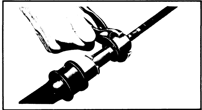
Fig. 1 Procedure for Removing Outer Bearing Cap Lock Nut
