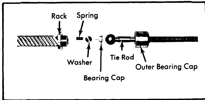
Fig.3 Exploded View of Ball Joint Assembly
