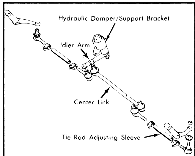
Fig. 2 Exploded View of Steering Linkage
