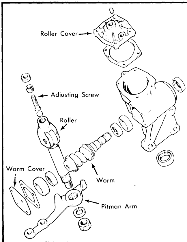
Fig. 1 Exploded View of Fiat Worm & Roller Steering Gear
