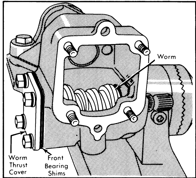
Fig. 3 View Showing Installation of Worm Thrust Cover and Location of Adjusting Shims
