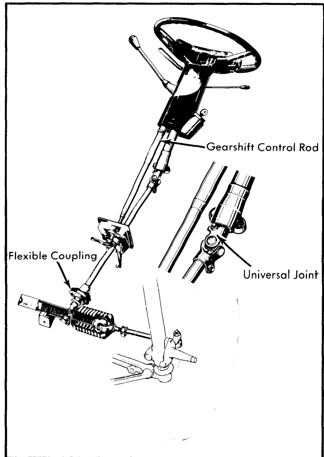
Fig. 2 Steering Column Assembly with Detail of Universal Joint Connection
