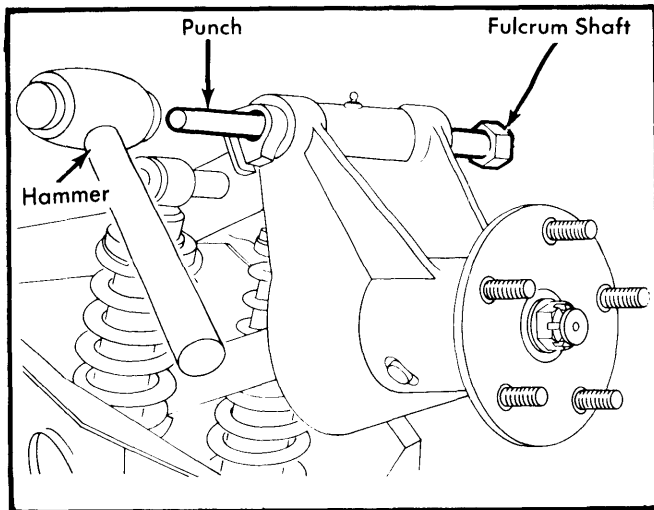
Fig. 3 Outer Fulcrum Shaft Removal
