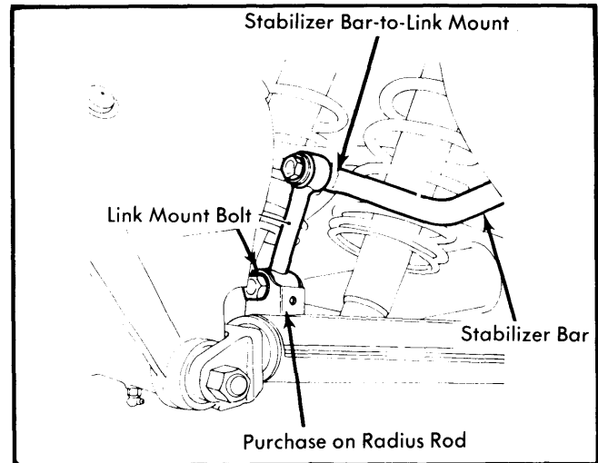
Fig. 4 Installed View of Stabilizer Bar and Connecting Link
