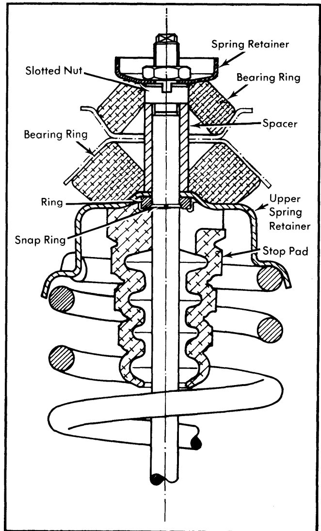
Fig. 1 Sectional View of Rear Suspension Coil Spring Assembly
