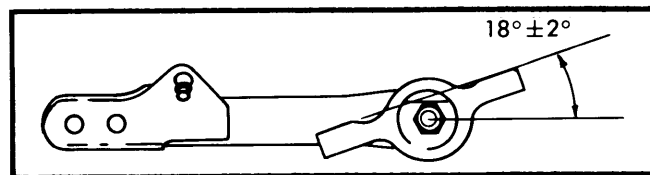
Fig. 3 View Showing Lower Control Arm-to-Bearing Angle
