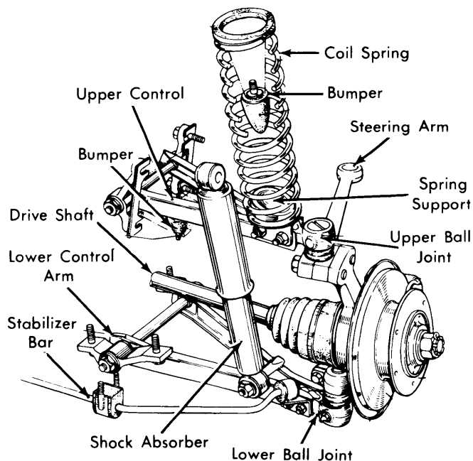
Fig. 1 Saab Front Suspension Assembly
