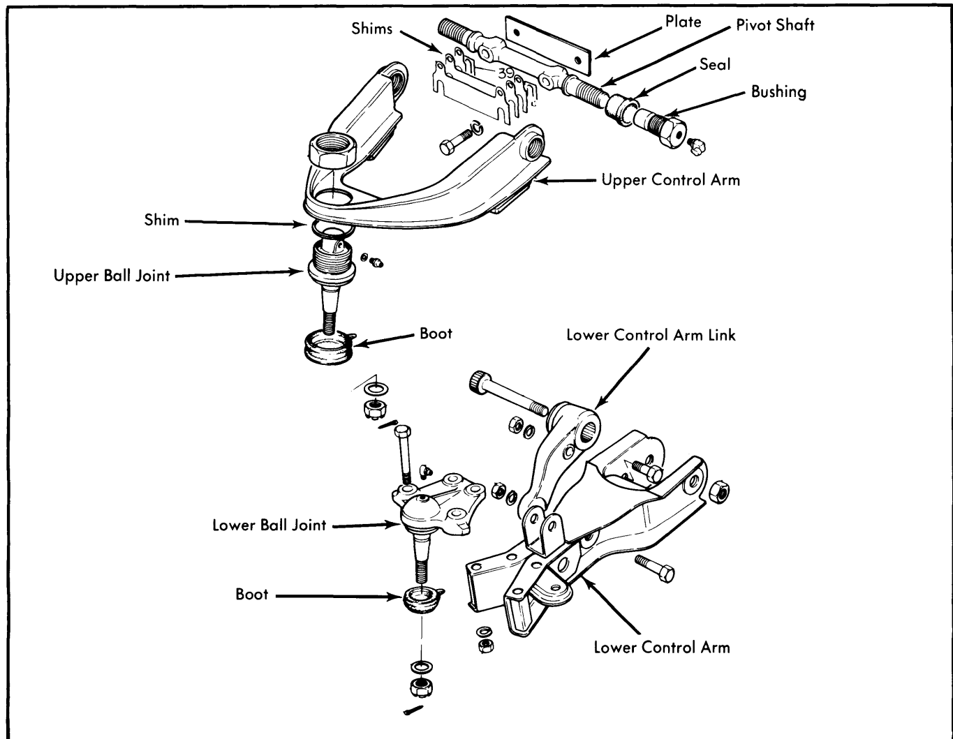
Fig. 3 Exploded View of LUV Front Suspension Assembly
