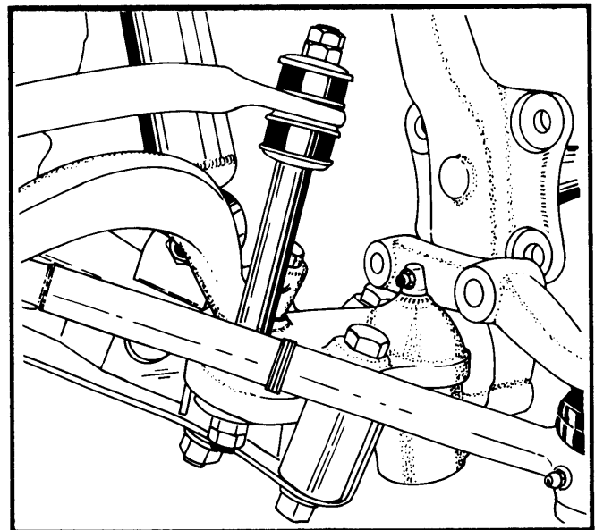
Fig. 2 Detail of Stabilizer Bar Link Bolt Installation
