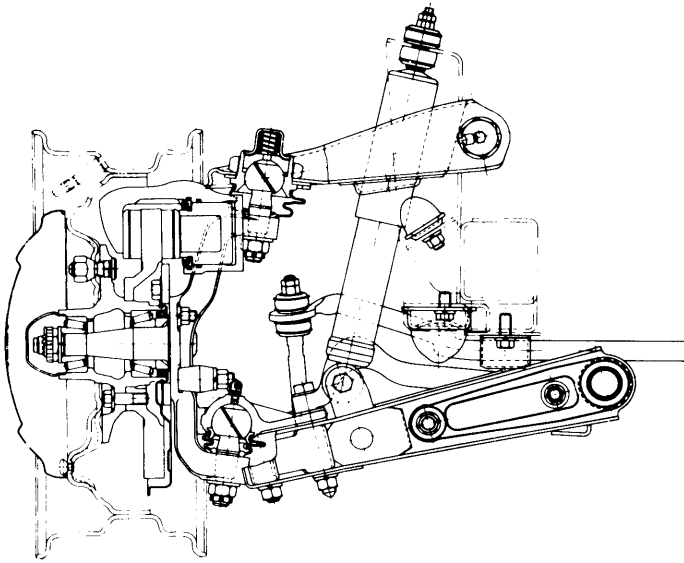
Fig. 1 Sectional View of Front Suspension Assembly
