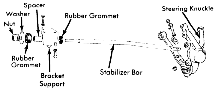
Fig. 3 Exploded View of Stabilizer Bar Assembly
