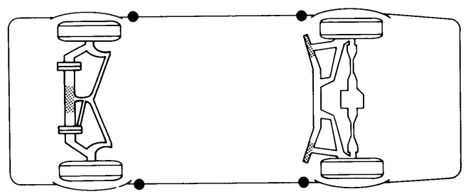
Volkswagen Type 1 and 2
