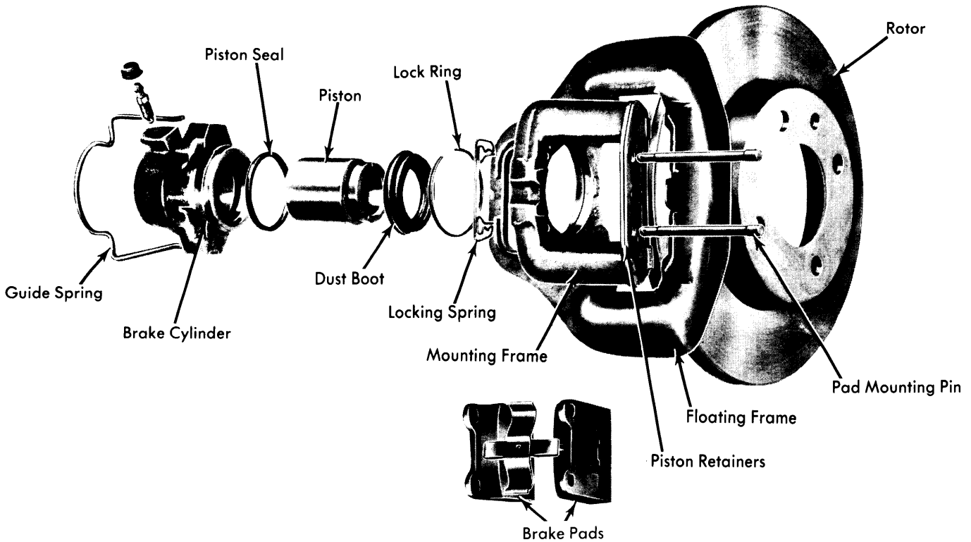
Fig. 5 Exploded View of ATE Disc Brake Assembly — Rabbit, Scirocco, Dasher
