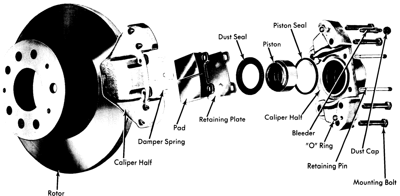
Fig. 2 Volkswagen Type 2 Front Disc Brake Assembly
