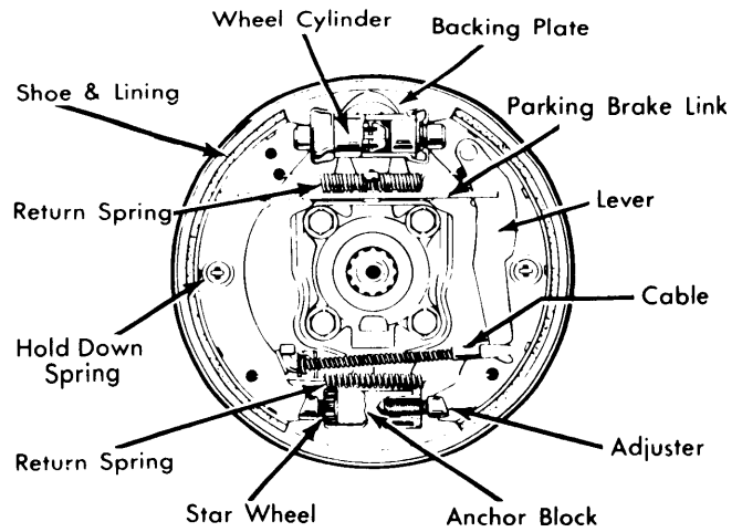
Fig. 4 Volkswagen Type 2 Rear Brake Assembly
