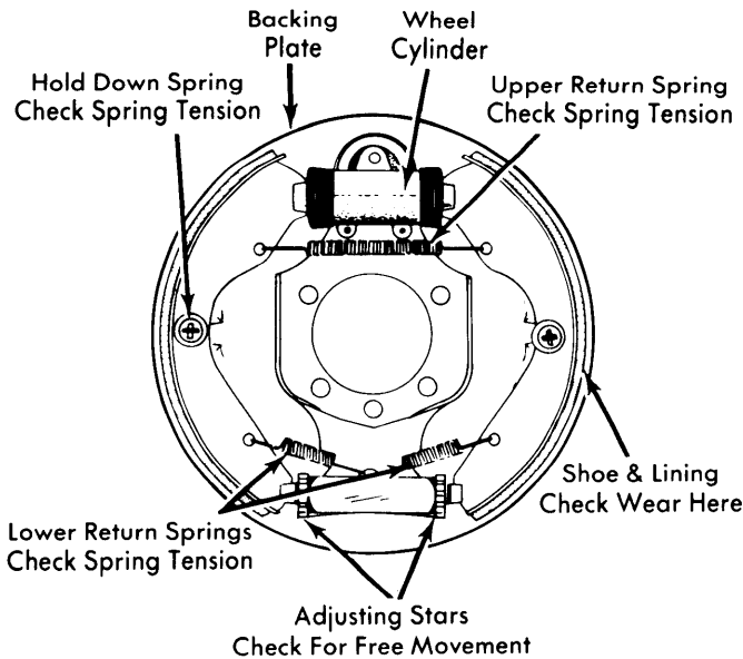
Fig. 3 Volkswagen Type 1 Front Brake Assembly
