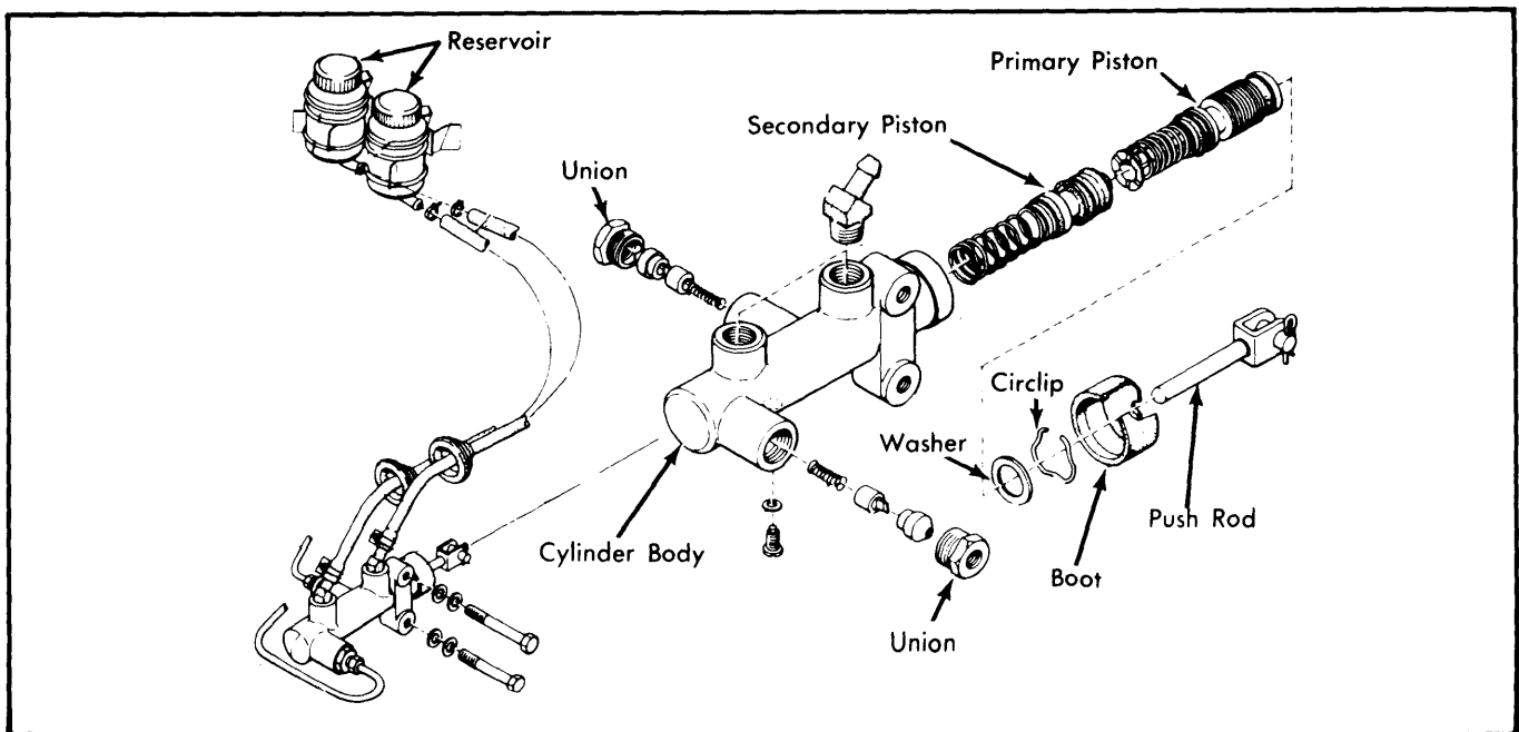
Fig. 4 Exploded View of Components in Tandem Master Cylinder
