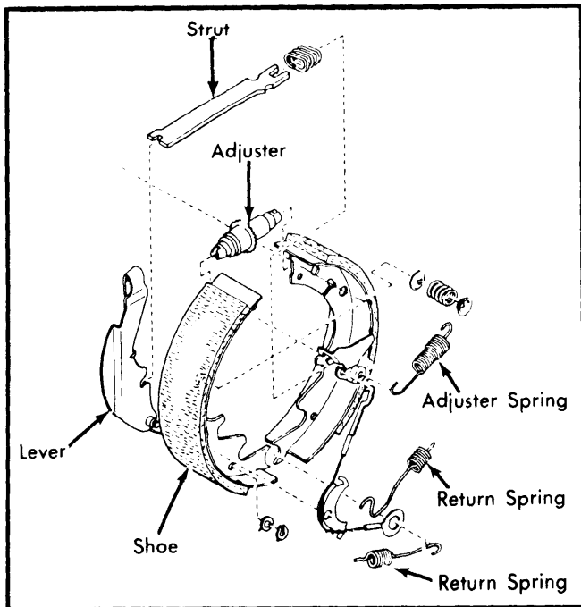
Fig. 2 Showing Components of Front Drum Brake Assembly
