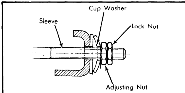
Fig. 1 Sectional View of Parking Brake Adjusting Nut and Cup Washer
