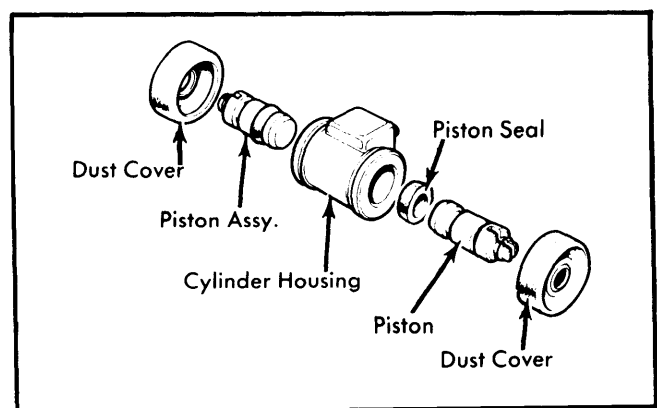
Fig. 3 Rear Wheel Cylinder Components
