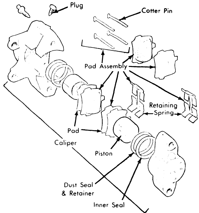
Fig. 2 Exploded View of Front Brake Caliper Assembly
