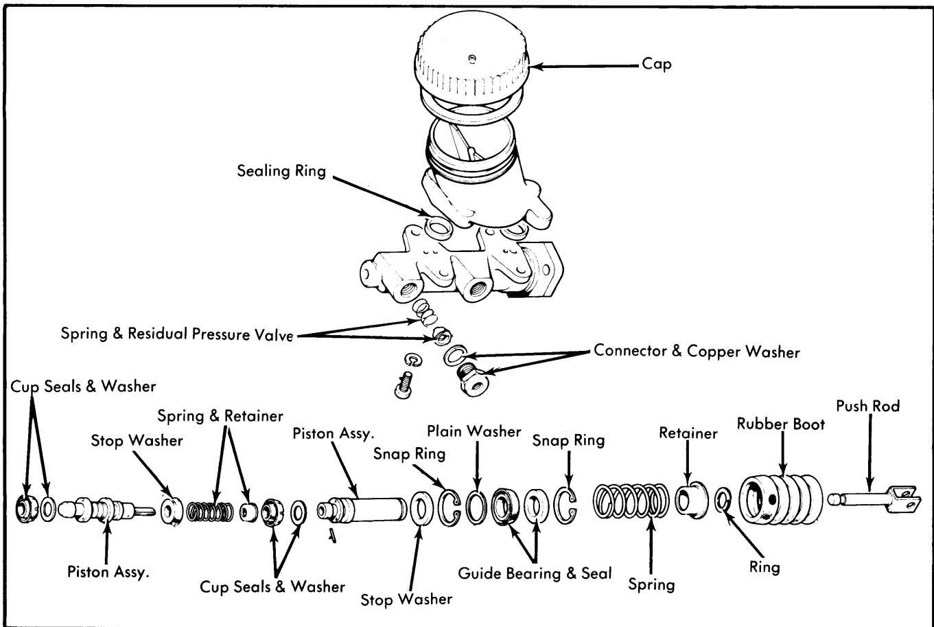
Fig. 4 Master Cylinder Reservoir, Body and Piston Assemblies
