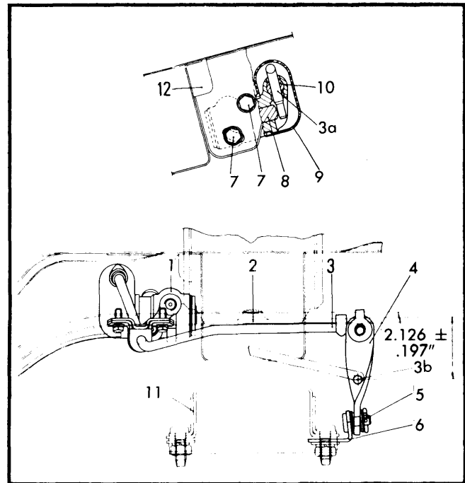
Fig. 1 Brake Pressure Regulator Measurement and Adjustment Points (128 Models)
