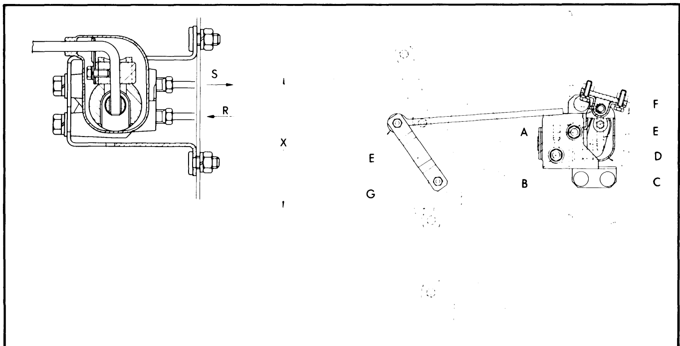
Fig. 2 Brake Pressure Regulator Measurement and Adjustment Points (124 Models)
