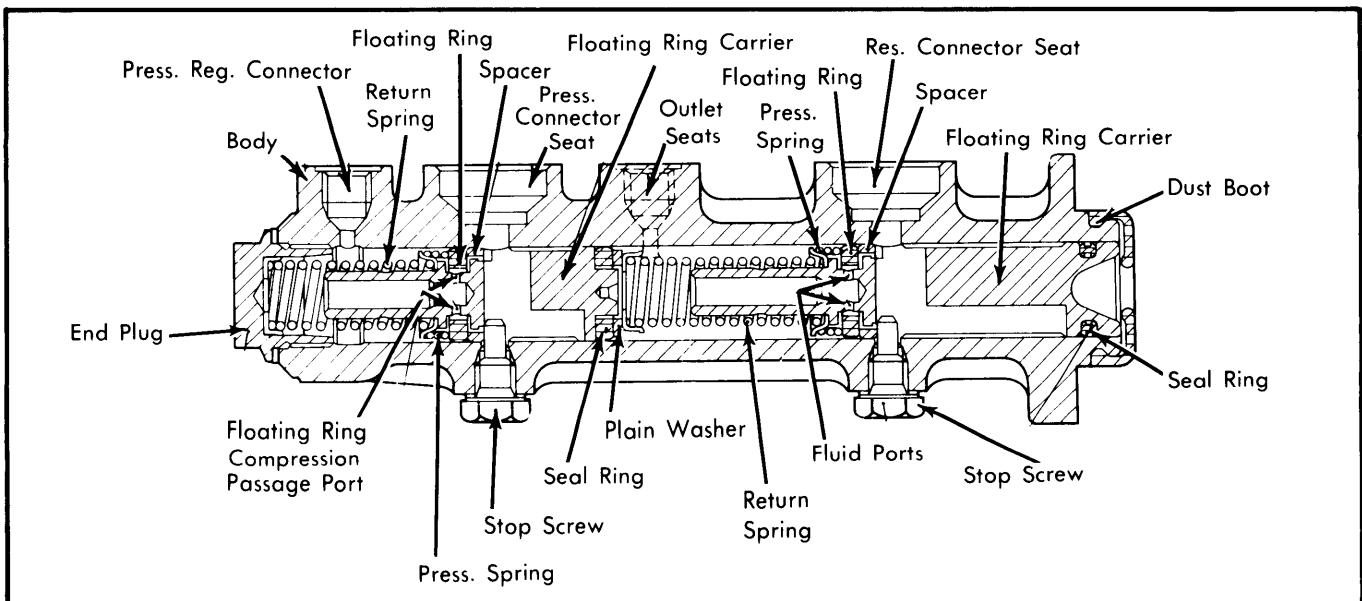
Fig. 10 Sectional View of Master Cylinder Assembly (128 Models)
