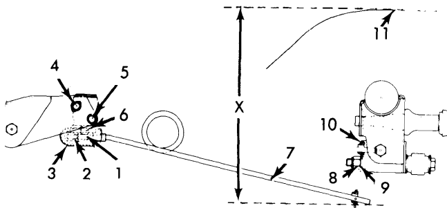
Fig. 3 Brake Pressure Regulator Measurement and Adjustment Points (131 Models)
