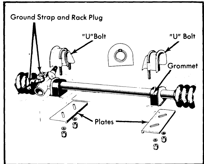
Fig. 2 Reassembly of Rack Rubber Grommets (TR6 and Spitfire)
