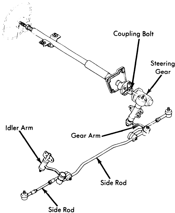
Fig. 1 Datsun Steering Gear Linkage B-210 Shown, Others Similar
