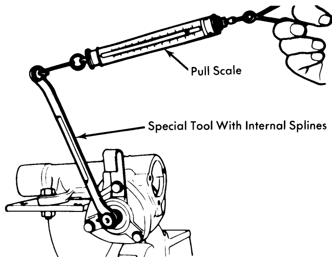
Fig. 3 Measuring Steering Gear Initial Turning Torque
