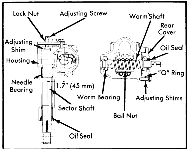
Fig. 2 Sectional View of Datsun Steering Gear
