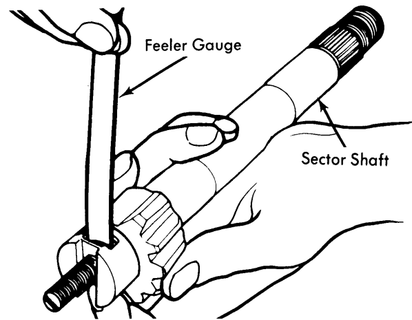
Fig. 4 Measuring Sector Shaft-to-Adjusting Screw End Play
