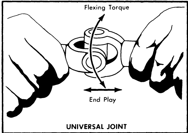
Fig. 2 Checking Universal Joint for Free Play
