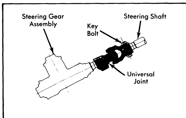
Fig. 2 Flexible Joint
