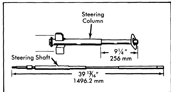
Fig. 3 Column and Shaft Measurements
