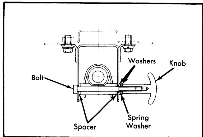
Fig. 2 Tilt Bracket Installation
