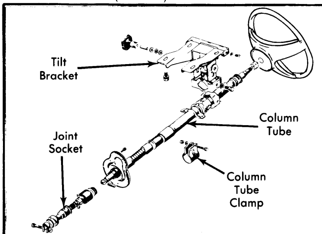
Fig. 1 Exploded View of Steering Column Assembly
