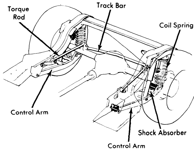
Fig. 1 Volvo Rear Suspension Assembly
