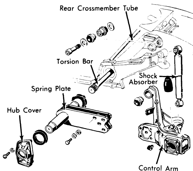
Fig. 1 Exploded View of Rear Suspension Assembly
